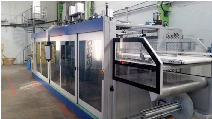
Figure 3: TM-800/4 FPCS Four station thermoforming line
